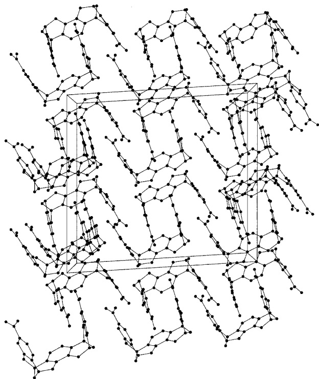
Figure 2. The unit cell of 17b
