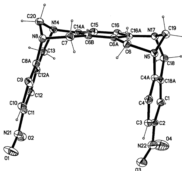
Figure 1. X-ray structure of 17b — an ORTEP view
